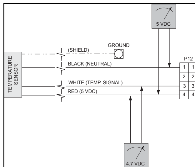
Figure 6.9 - Temperature Sensor Harness
