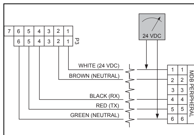
Figure 6.3 - MDB Harness
